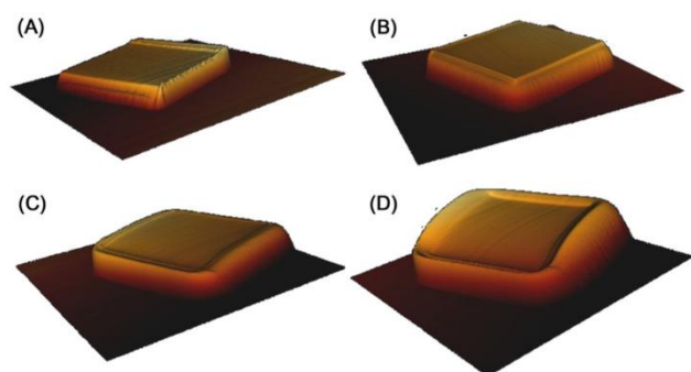
Figure 2. Topography of linear polysiloxane structures post-exposure to electron beam doses of (a) 130 \mu\text{C}/\text{cm}^2 , (b) 542 \mu\text{C}/\text{cm}^2 , (c) 2.26 \text{ mC}/\text{cm}^2 , and (d) 9.39 \text{ mC}/\text{cm}^2
