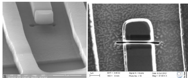
Figure 2 A single line pass made through 2 µm thick silicon.
